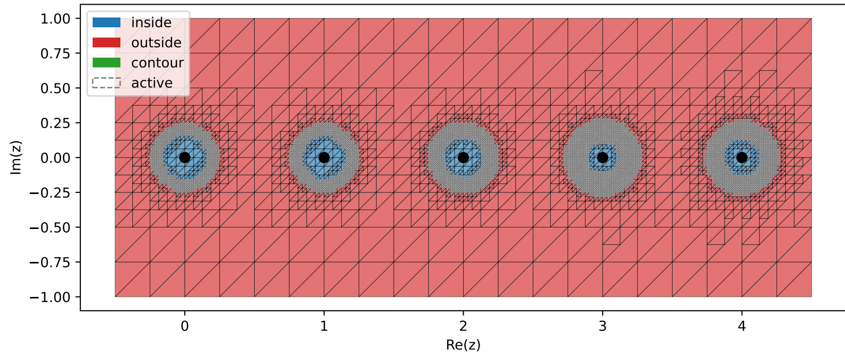
Outer-loop classification: sweep 3
